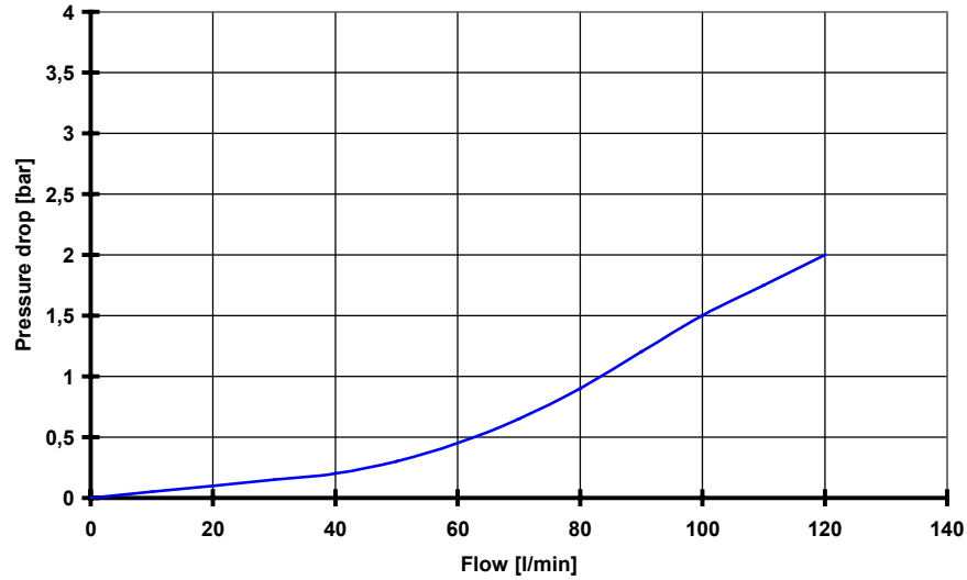
RVM/UM, Pressure drop for water at 20 °C
